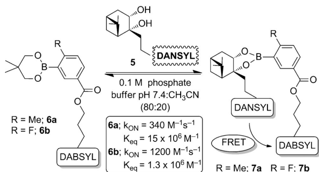
Figure 2. Kinetic analysis using a fluorescence quenching experiment to measure the initial rate of boronate formation. Reported k_{\text{ON}} and K_{\text{eq}} are the average of at least three measurements. [16]
